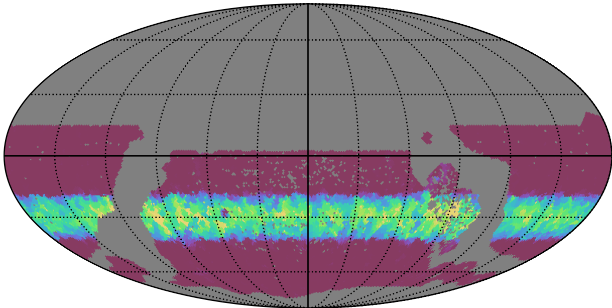
too_100_4v3.4_10yrs WFD u band: Min normairmass
