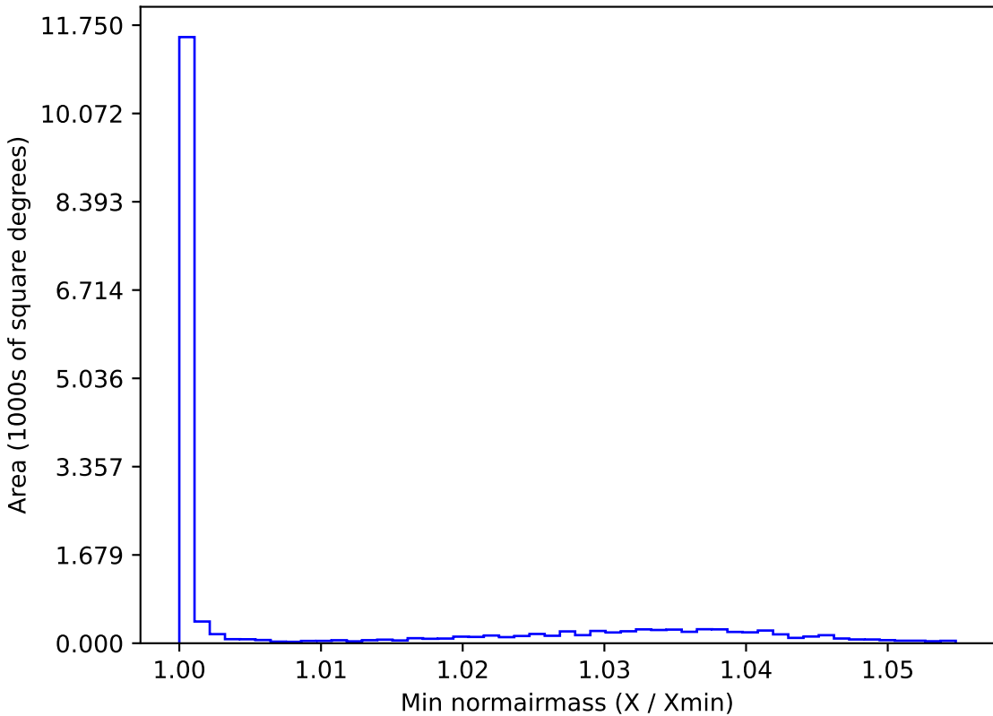
too_100_4v3.4_10yrs WFD u band: Min normairmass
