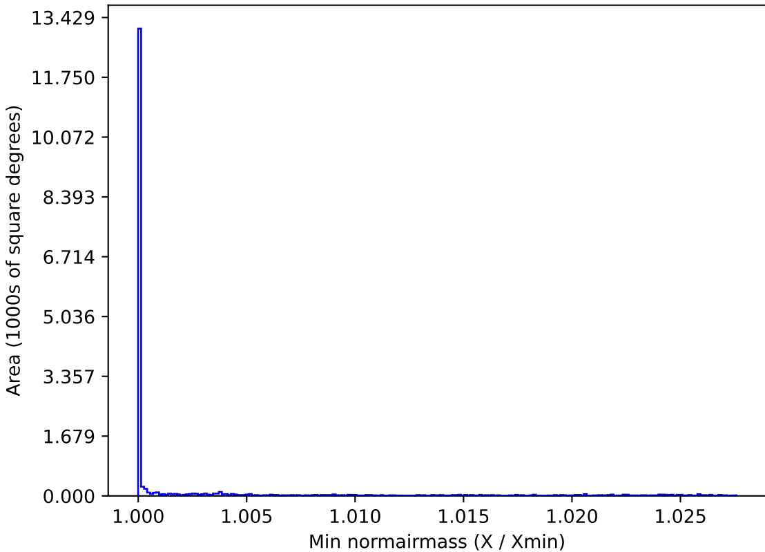
too_100_4v3.4_10yrs WFD all bands: Min normairmass
