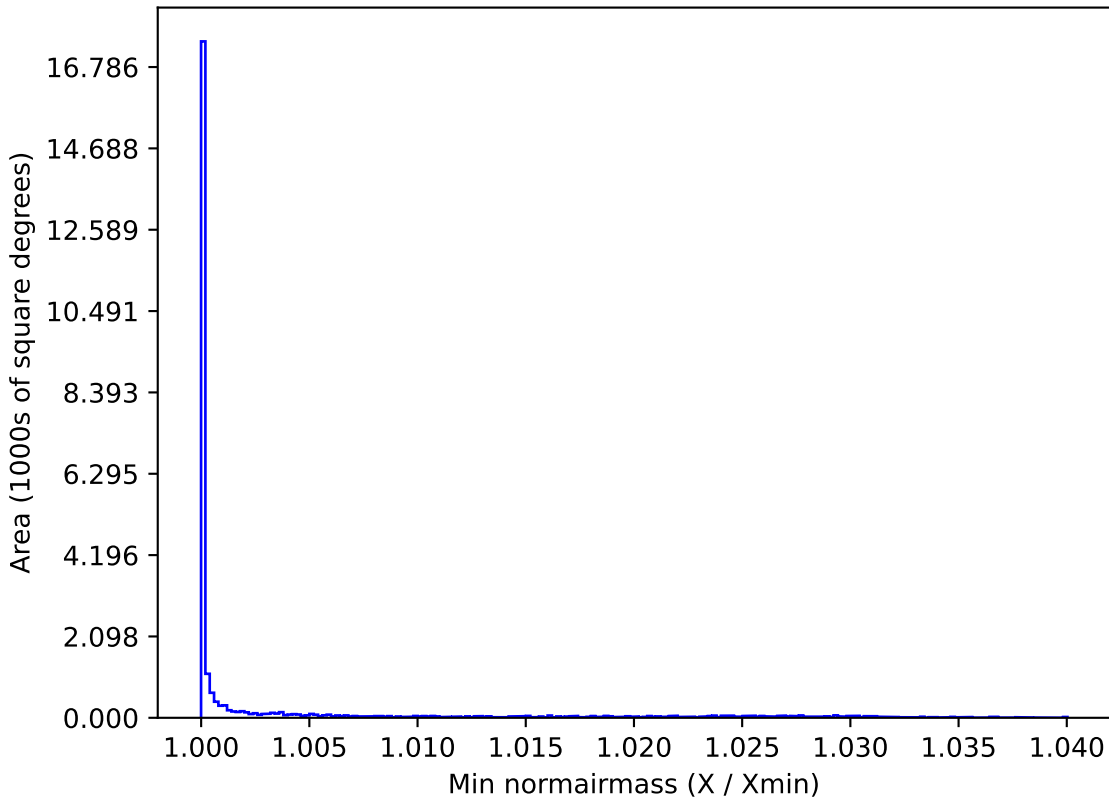
too_100_4v3.4_10yrs All sky z band: Min normairmass
