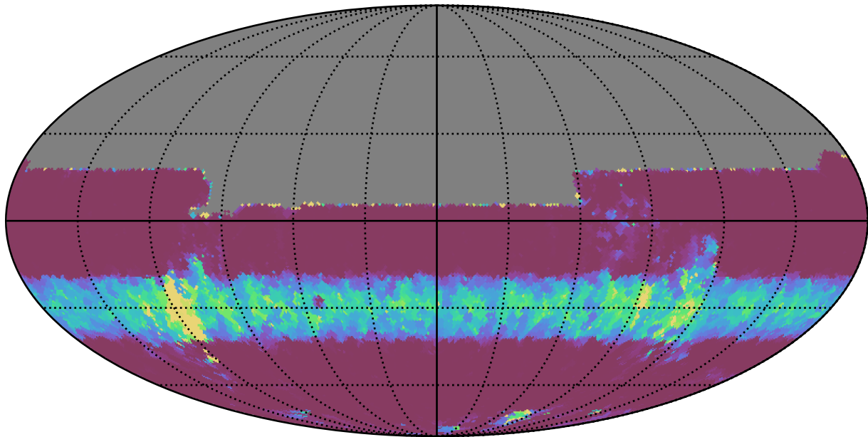
too_100_4v3.4_10yrs All sky u band: Min normairmass
