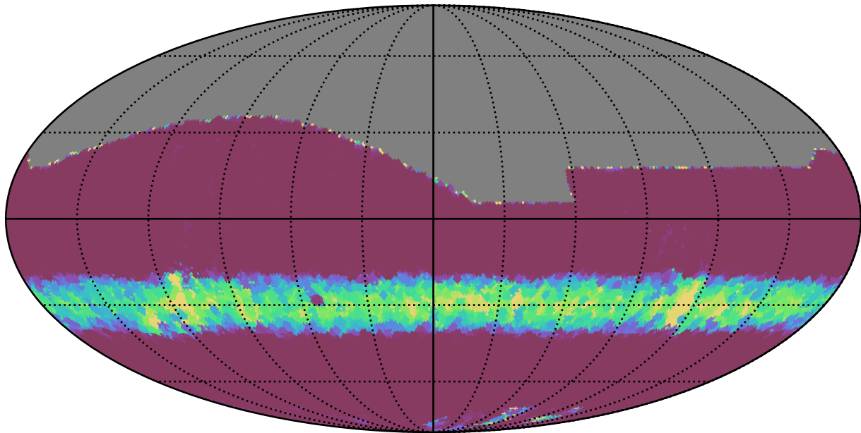
too_100_4v3.4_10yrs All sky r band: Min normairmass
