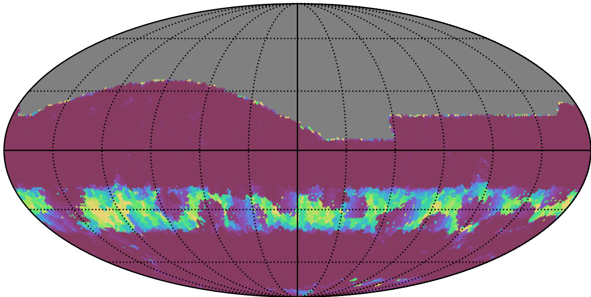
too_100_4v3.4_10yrs All sky g band: Min normairmass
