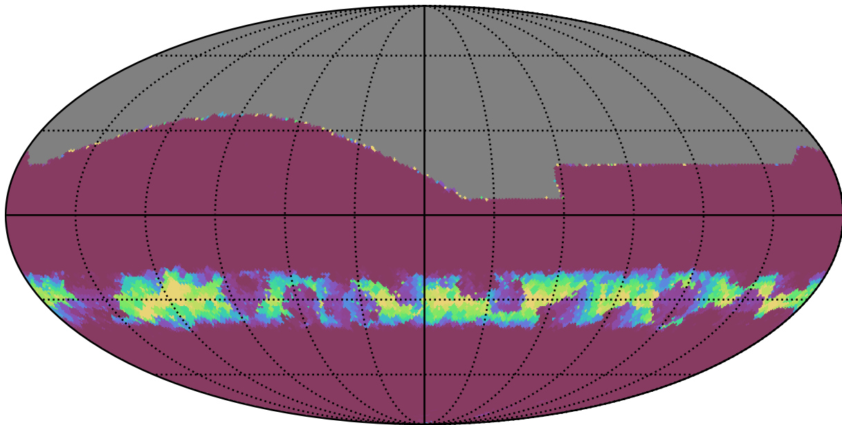
too_100_4v3.4_10yrs All sky all bands: Min normairmass
