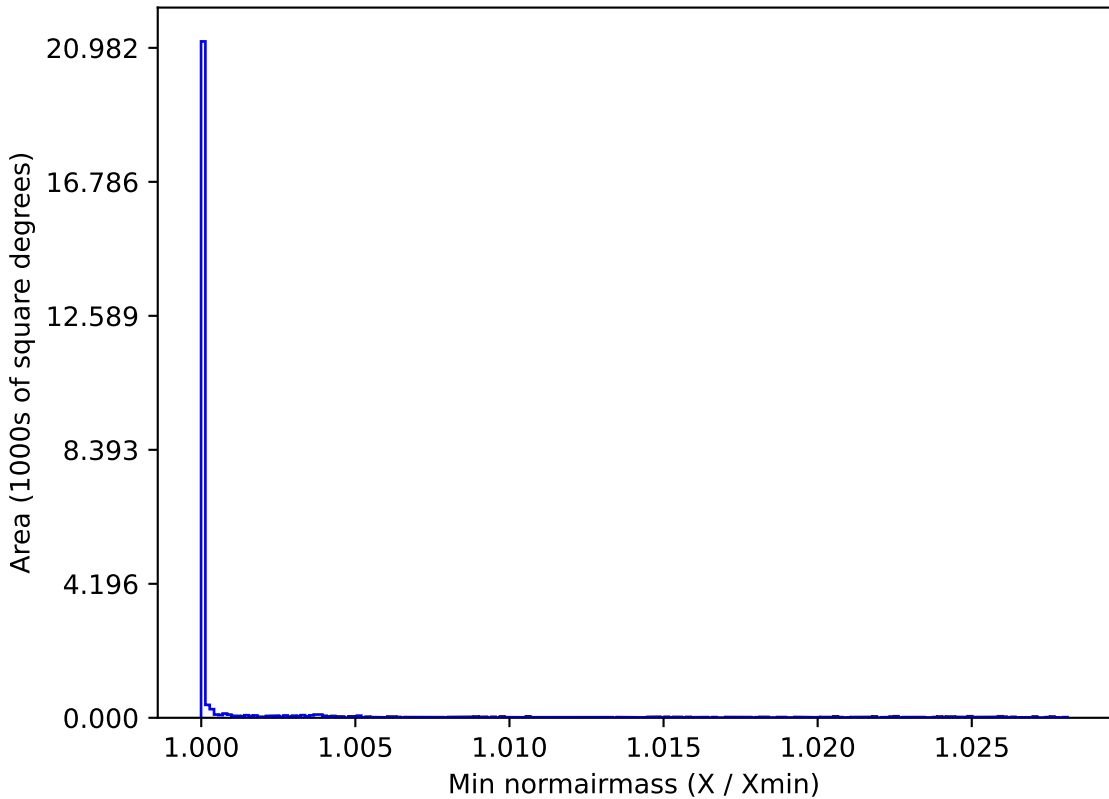
too_100_4v3.4_10yrs All sky all bands: Min normairmass
