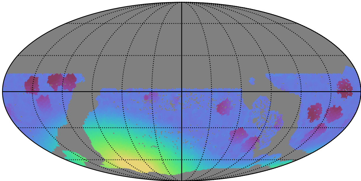
too_100_4v3.4_10yrs WFD z band: Min moonDistance
