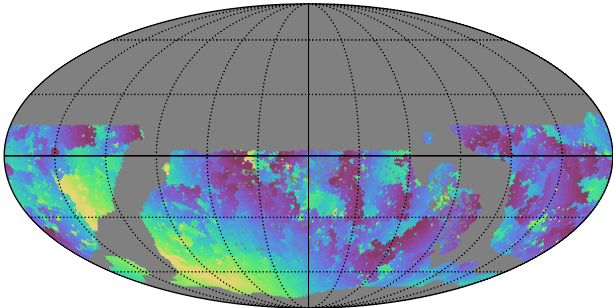
too_100_4v3.4_10yrs WFD u band: Min moonDistance
