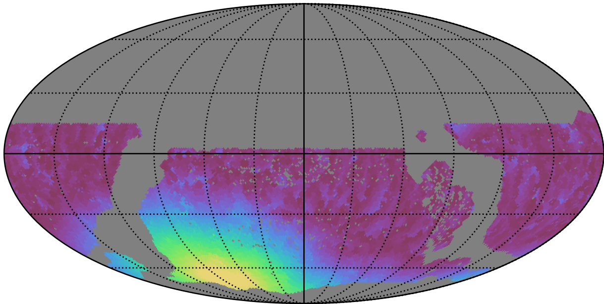
too_100_4v3.4_10yrs WFD r band: Min moonDistance
