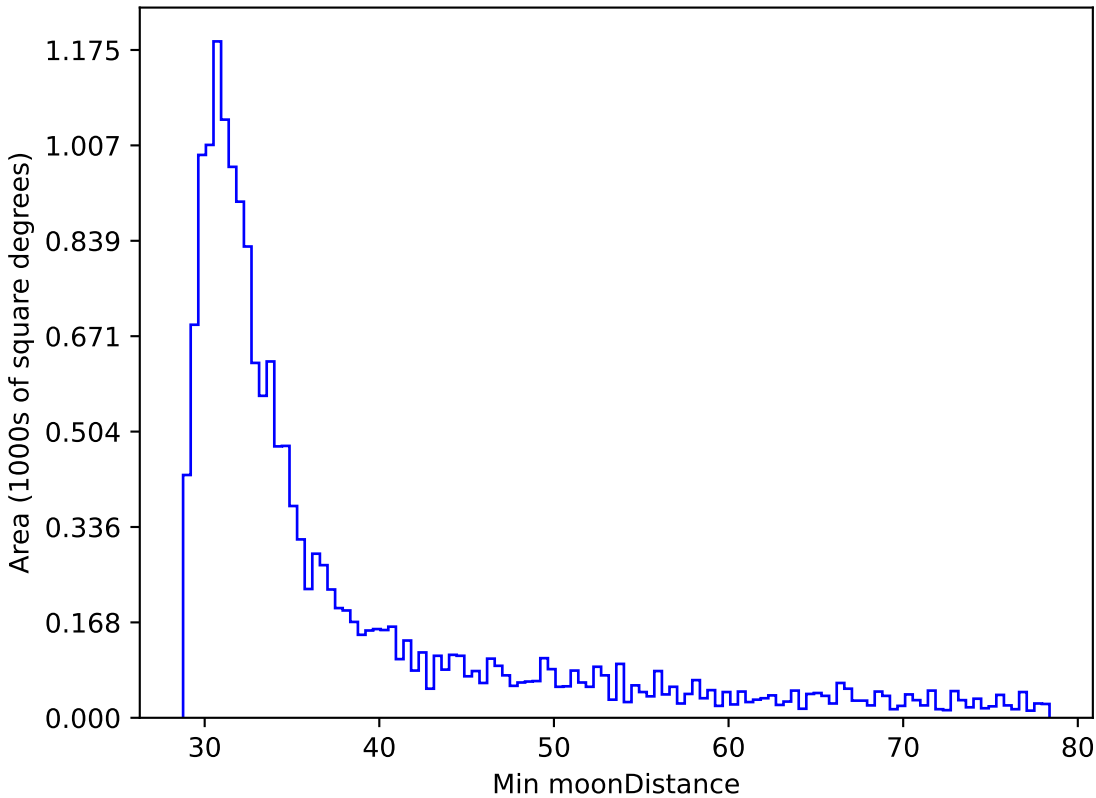
too_100_4v3.4_10yrs WFD r band: Min moonDistance
