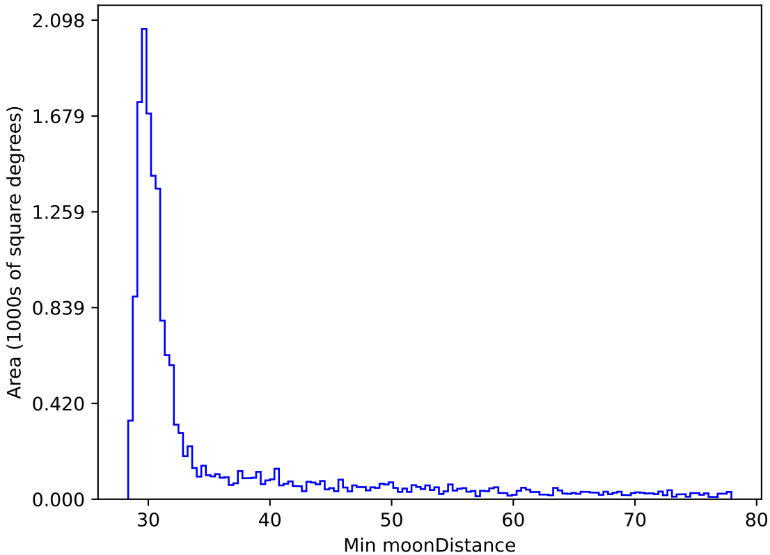
too_100_4v3.4_10yrs WFD i band: Min moonDistance
