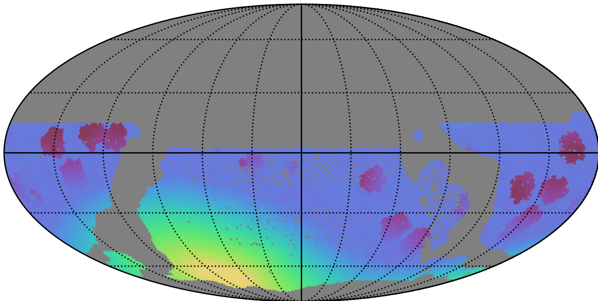
too_100_4v3.4_10yrs WFD all bands: Min moonDistance
