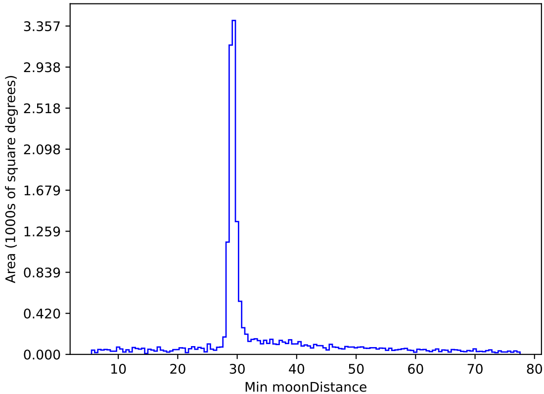
too_100_4v3.4_10yrs WFD all bands: Min moonDistance
