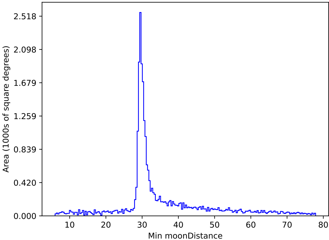
too_100_4v3.4_10yrs All sky z band: Min moonDistance
