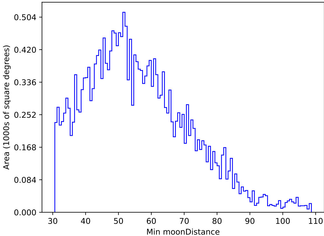
too_100_4v3.4_10yrs All sky u band: Min moonDistance
