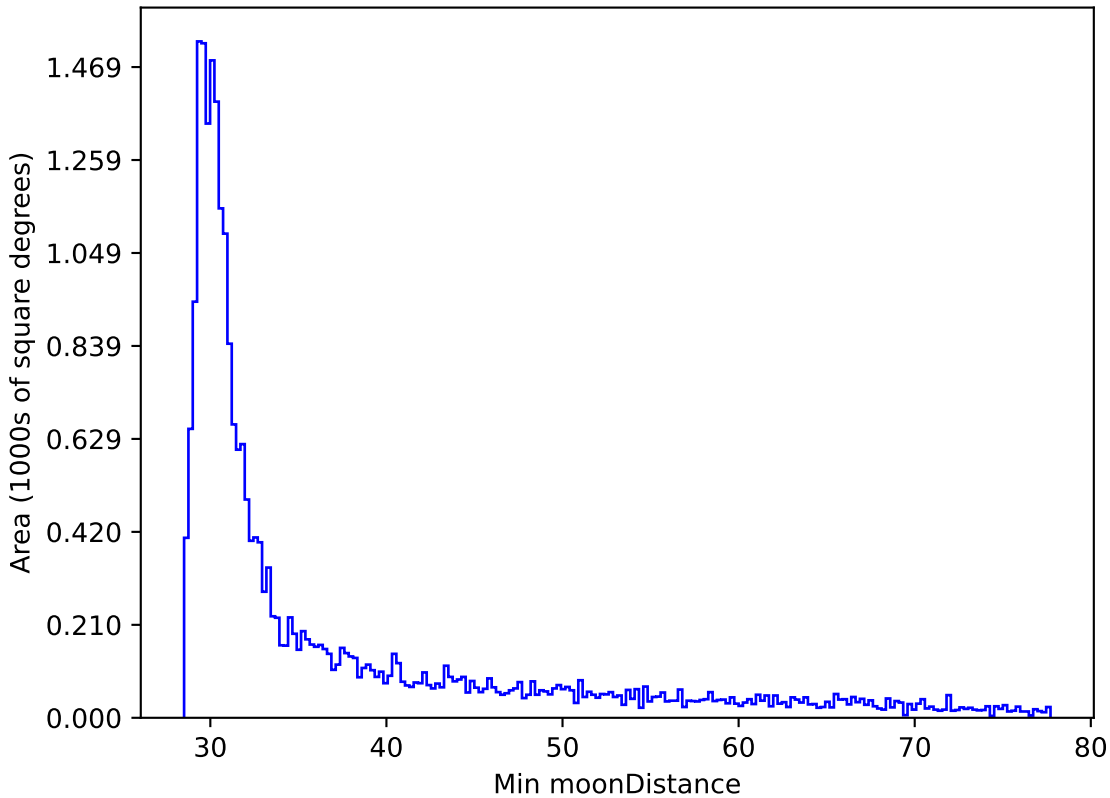
too_100_4v3.4_10yrs All sky i band: Min moonDistance
