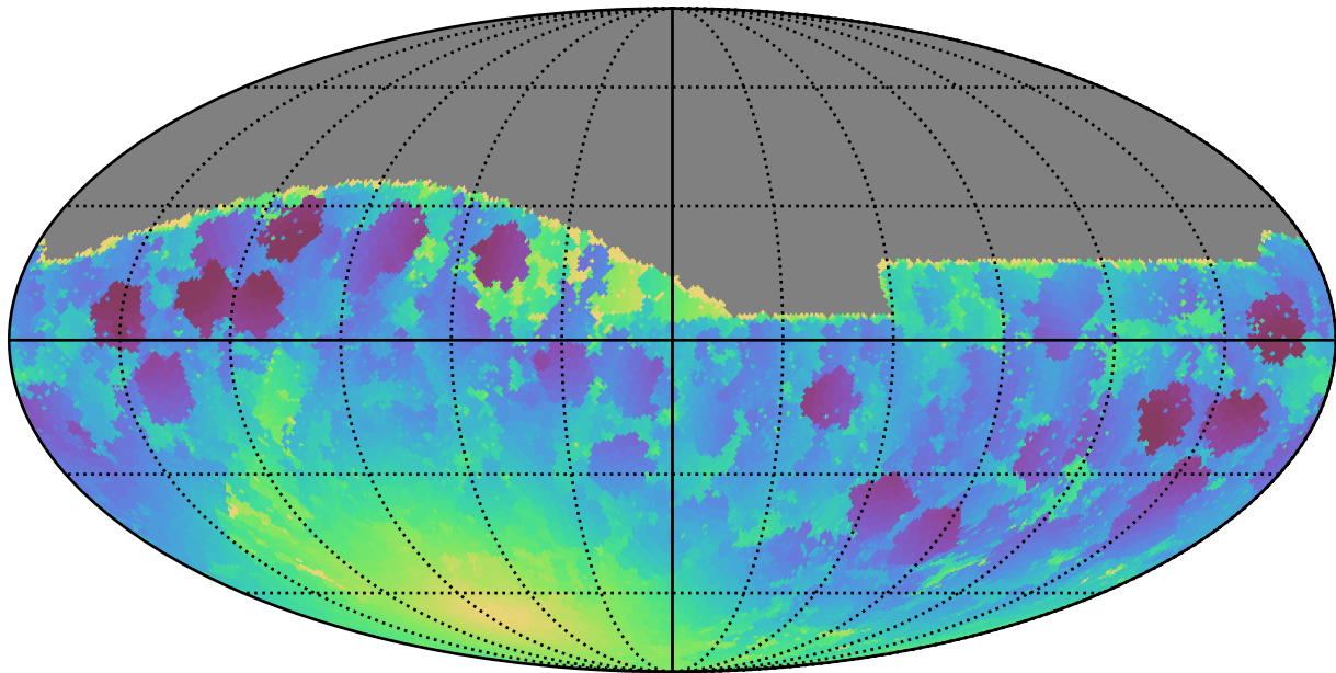
too_100_4v3.4_10yrs All sky g band: Min moonDistance
