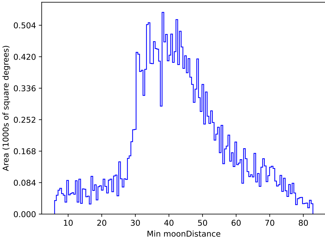
too_100_4v3.4_10yrs All sky g band: Min moonDistance
