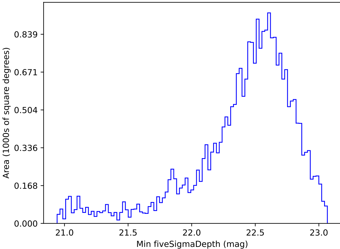
too_100_4v3.4_10yrs Yr 1 z band: Min fiveSigmaDepth
