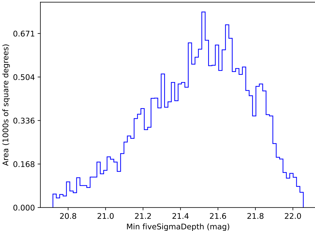
too_100_4v3.4_10yrs Yr 1 y band: Min fiveSigmaDepth
