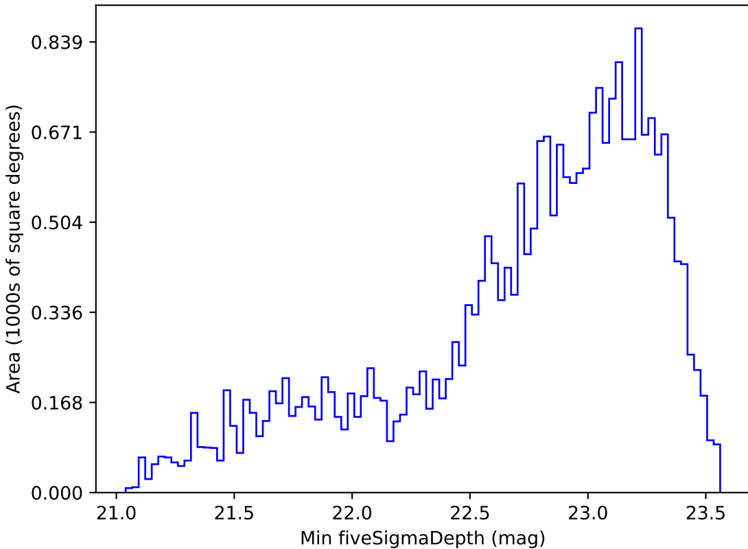
too_100_4v3.4_10yrs Yr 1 i band: Min fiveSigmaDepth
