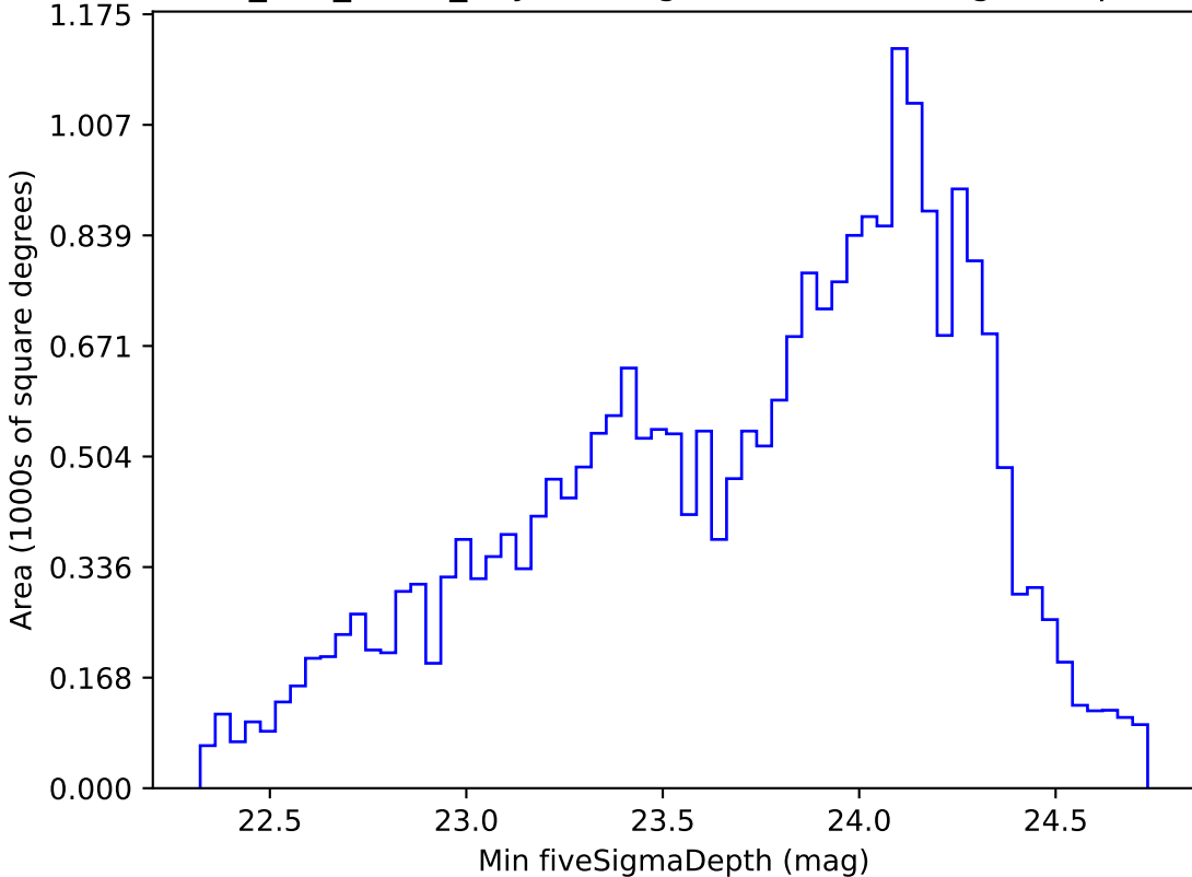
too_100_4v3.4_10yrs Yr 1 g band: Min fiveSigmaDepth
