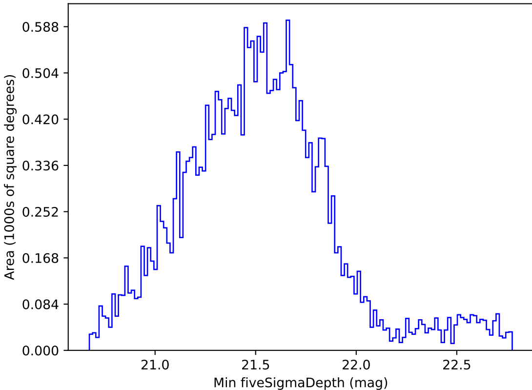
too_100_4v3.4_10yrs Yr 1 all bands: Min fiveSigmaDepth
