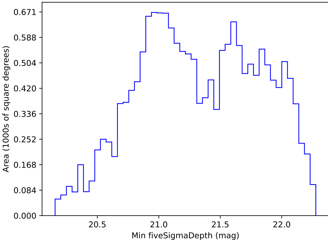
too_100_4v3.4_10yrs WFD z band: Min fiveSigmaDepth
