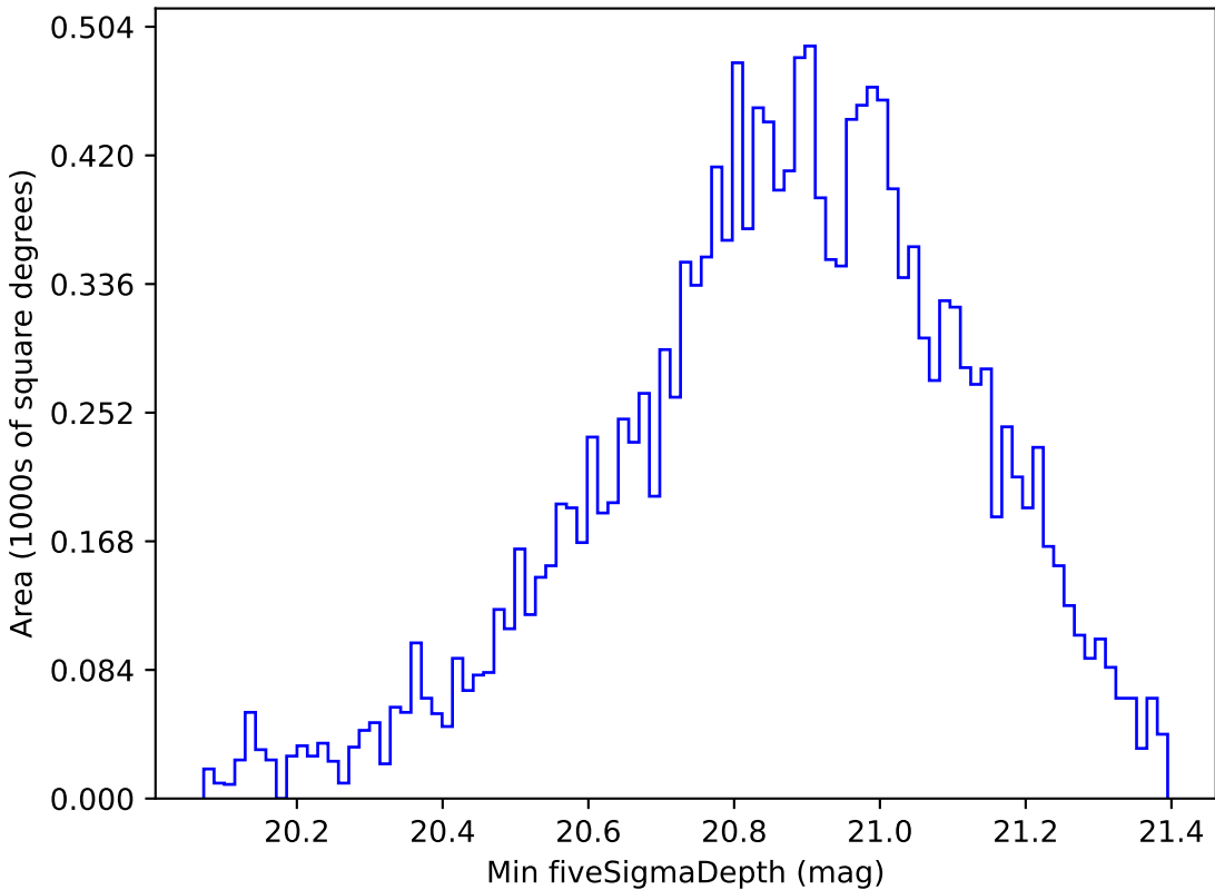
too_100_4v3.4_10yrs WFD y band: Min fiveSigmaDepth
