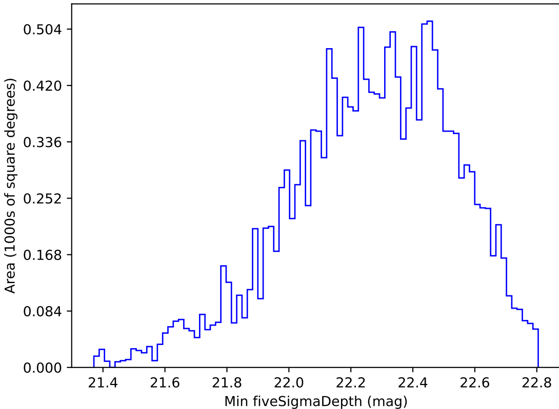
too_100_4v3.4_10yrs WFD u band: Min fiveSigmaDepth
