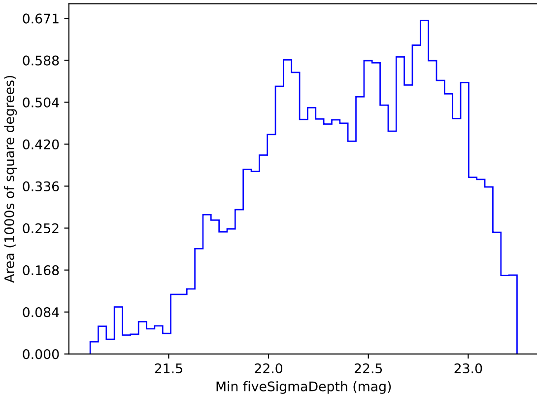
too_100_4v3.4_10yrs WFD r band: Min fiveSigmaDepth
