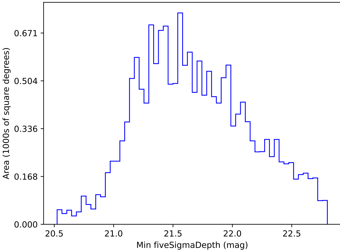
too_100_4v3.4_10yrs WFD i band: Min fiveSigmaDepth
