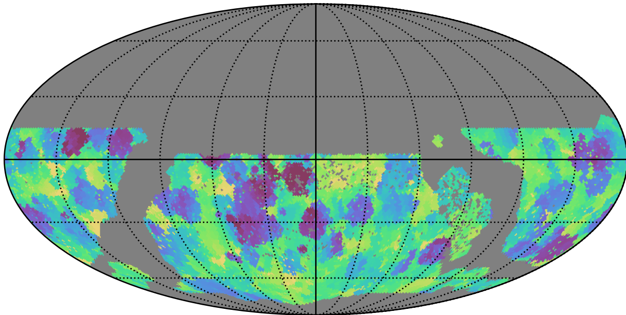
too_100_4v3.4_10yrs WFD g band: Min fiveSigmaDepth
