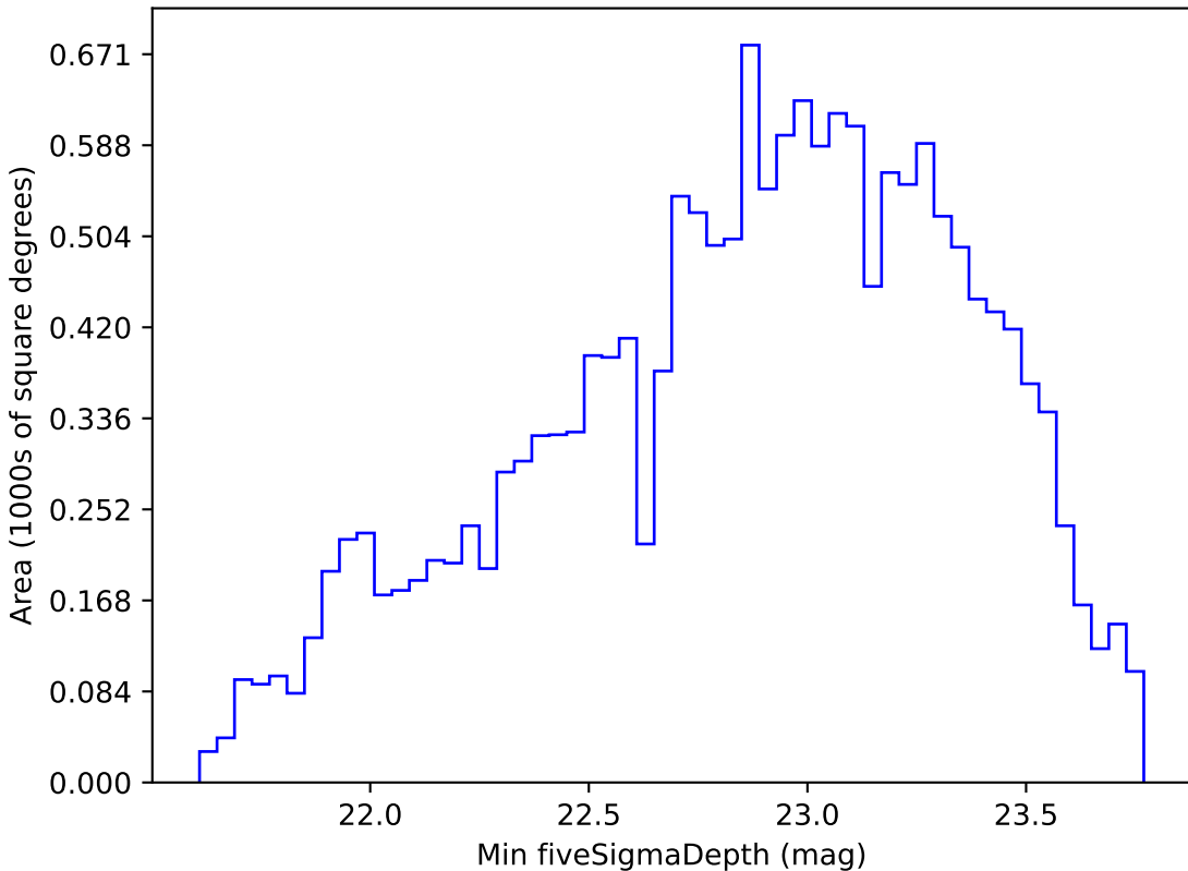
too_100_4v3.4_10yrs WFD g band: Min fiveSigmaDepth
