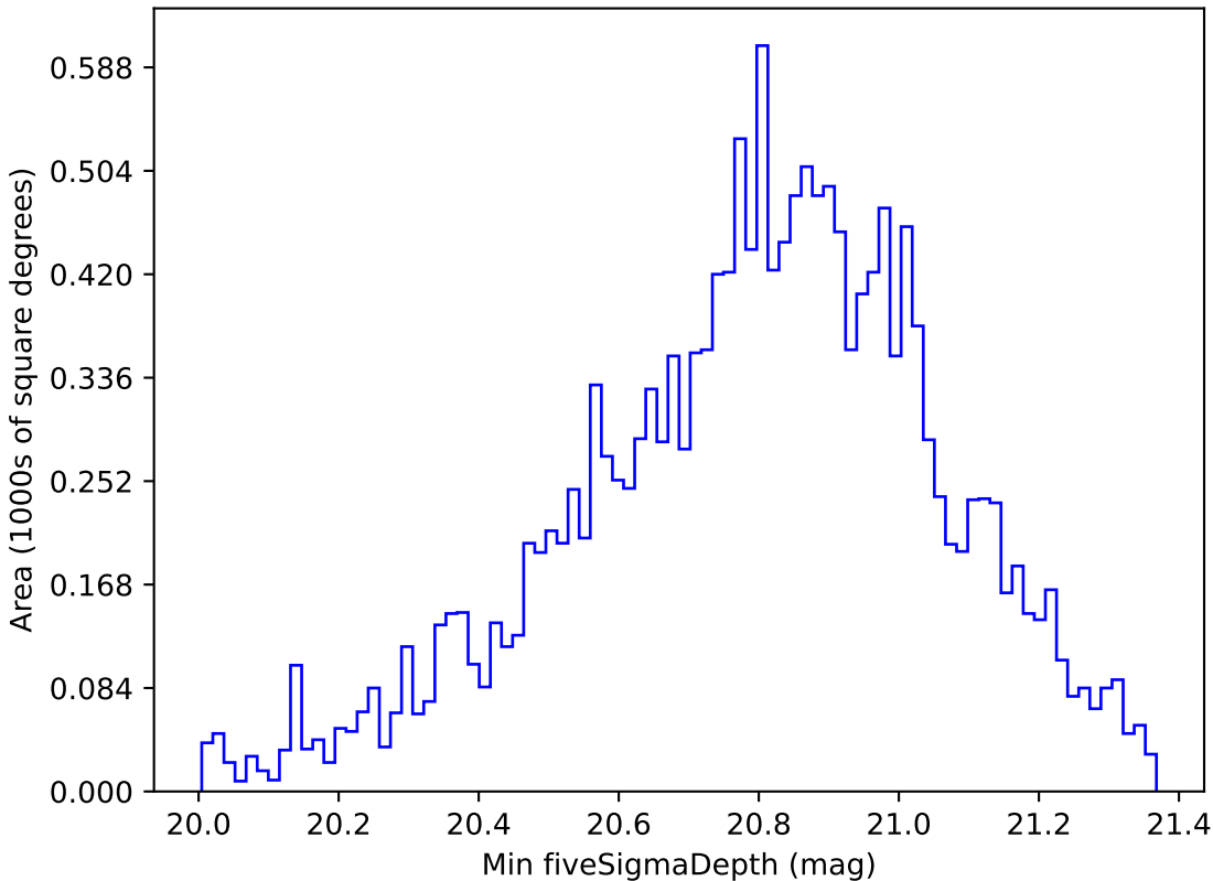
too_100_4v3.4_10yrs WFD all bands: Min fiveSigmaDepth
