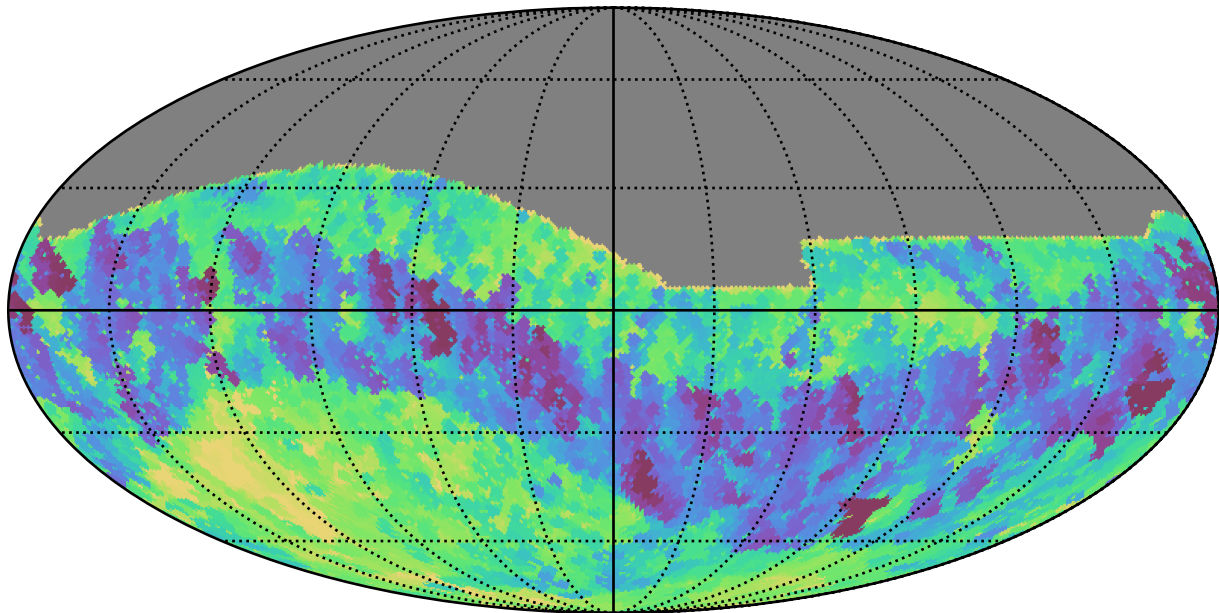
too_100_4v3.4_10yrs All sky z band: Min fiveSigmaDepth
