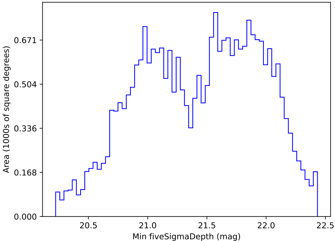
too_100_4v3.4_10yrs All sky z band: Min fiveSigmaDepth
