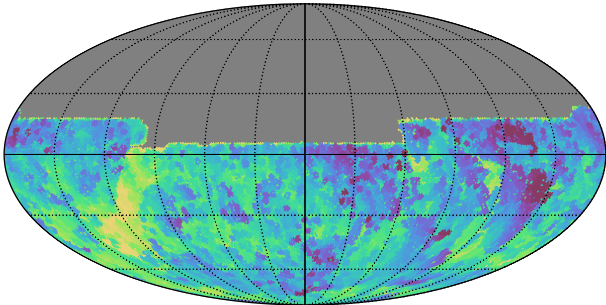
too_100_4v3.4_10yrs All sky y band: Min fiveSigmaDepth
