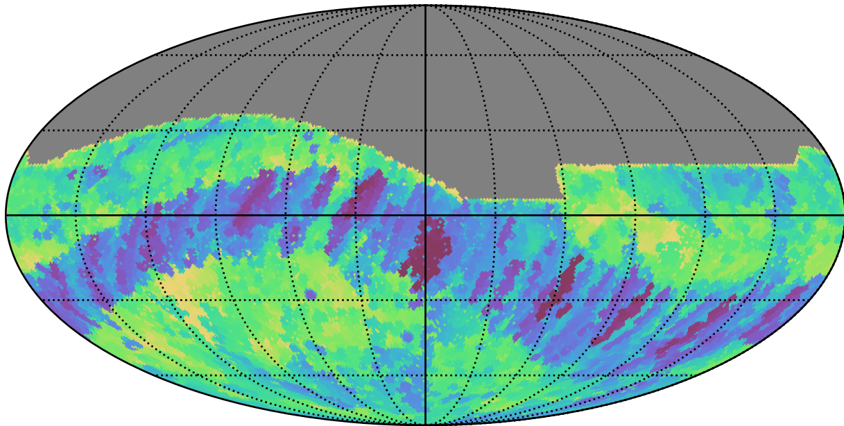
too_100_4v3.4_10yrs All sky r band: Min fiveSigmaDepth
