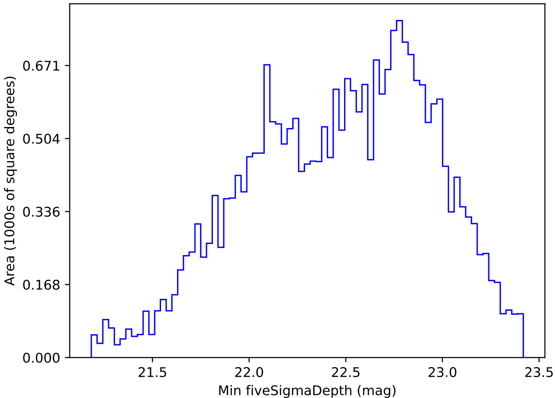
too_100_4v3.4_10yrs All sky r band: Min fiveSigmaDepth
