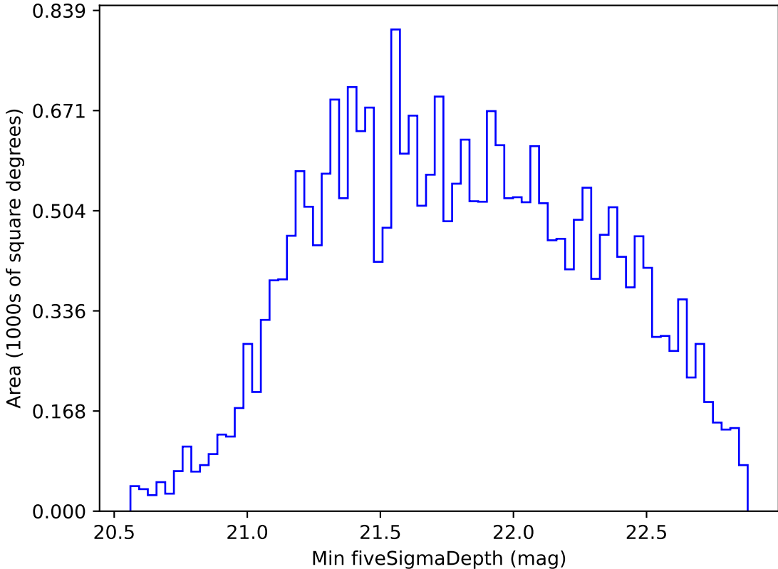
too_100_4v3.4_10yrs All sky i band: Min fiveSigmaDepth
