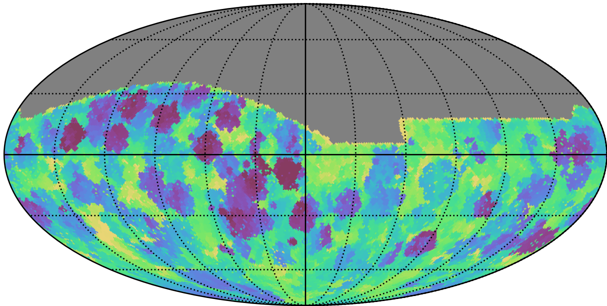
too_100_4v3.4_10yrs All sky g band: Min fiveSigmaDepth
