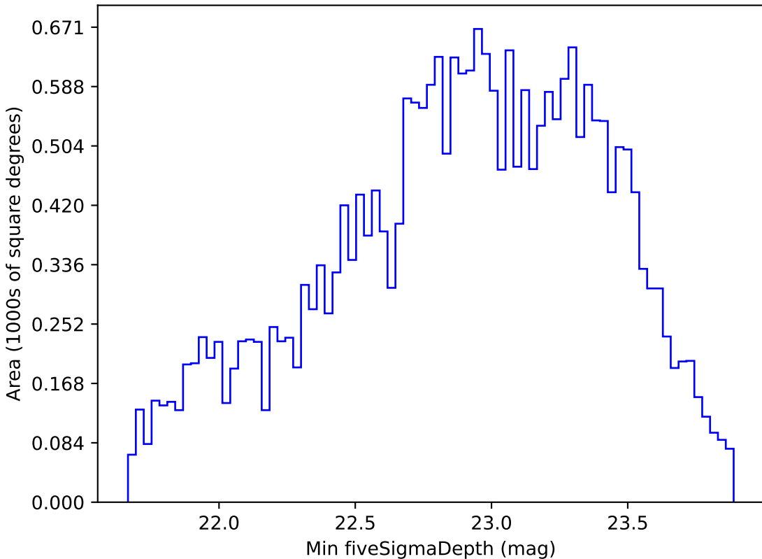
too_100_4v3.4_10yrs All sky g band: Min fiveSigmaDepth
