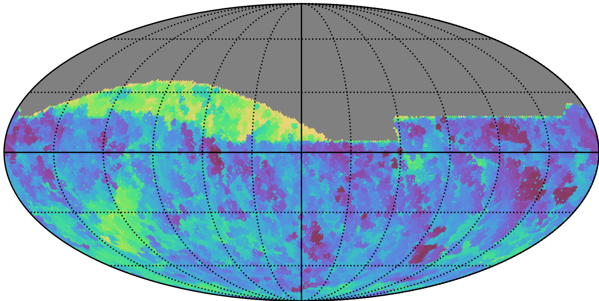
too_100_4v3.4_10yrs All sky all bands: Min fiveSigmaDepth
