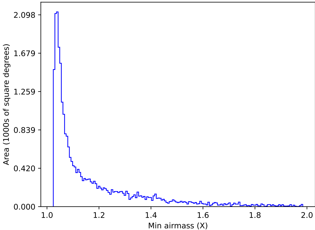
too_100_4v3.4_10yrs Yr 1 z band: Min airmass
