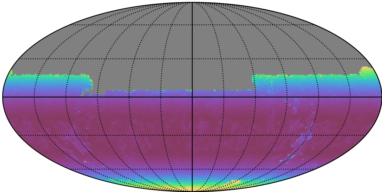
too_100_4v3.4_10yrs Yr 1 y band: Min airmass
