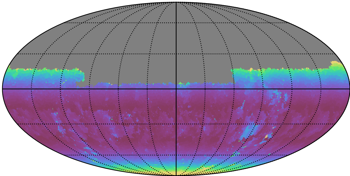
too_100_4v3.4_10yrs Yr 1 u band: Min airmass
