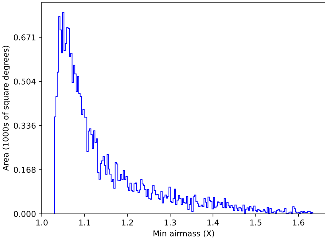
too_100_4v3.4_10yrs Yr 1 u band: Min airmass
