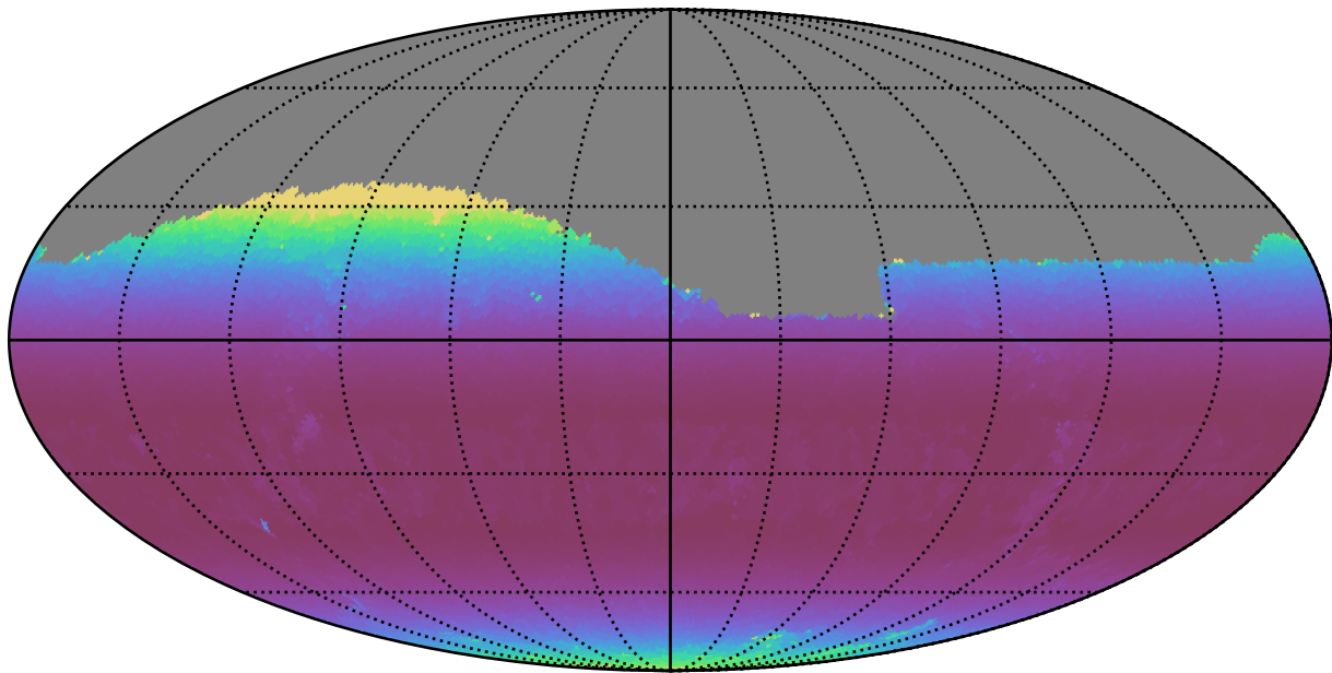
too_100_4v3.4_10yrs Yr 1 r band: Min airmass
