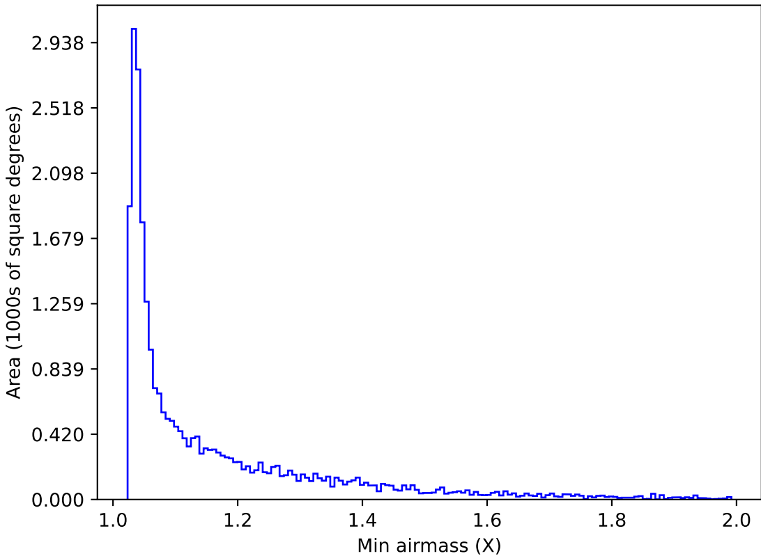
too_100_4v3.4_10yrs Yr 1 r band: Min airmass
