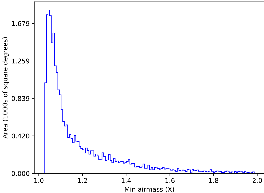
too_100_4v3.4_10yrs Yr 1 g band: Min airmass
